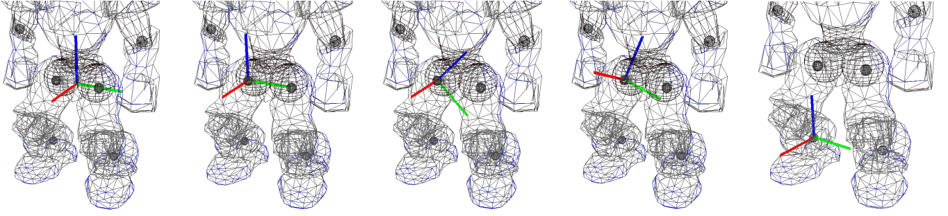
Fig. 3. Visualization of coordinate frames used in the inverse kinematic. From left to right: Torso , Hip , HipOrth , Thigh , Foot . The x -axis is shown in red, the y -axis in green, and the z -axis in blue.
