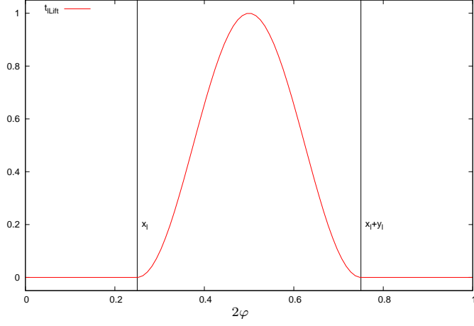
Fig. 5. The trajectory t_{lLift} that is used for foot lifting. t_{rLift} is similar to t_{lLift} except that it is shifted one half-phase to the right.
