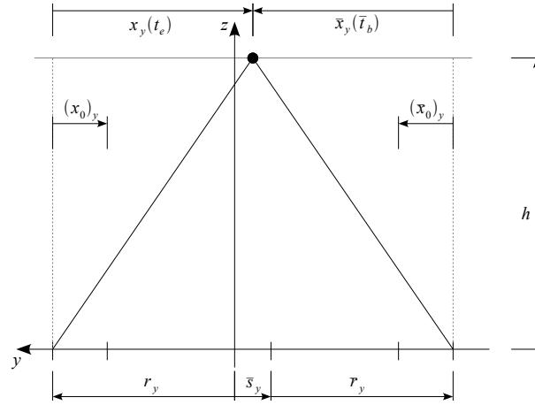
Fig. 5. Two facing inverted pendulums used to cover step size \bar{s}_y .
